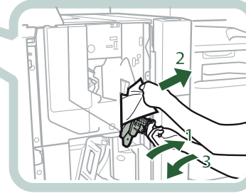
Saddle Stitcher Unit (p. 129)
